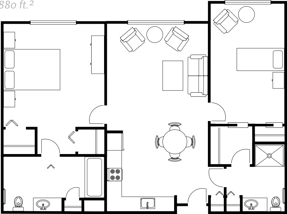
TWO BEDROOM 880 ft. 2
